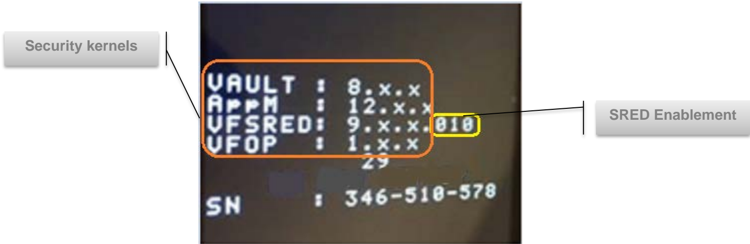
Figure 3, Boot Splash Screen
