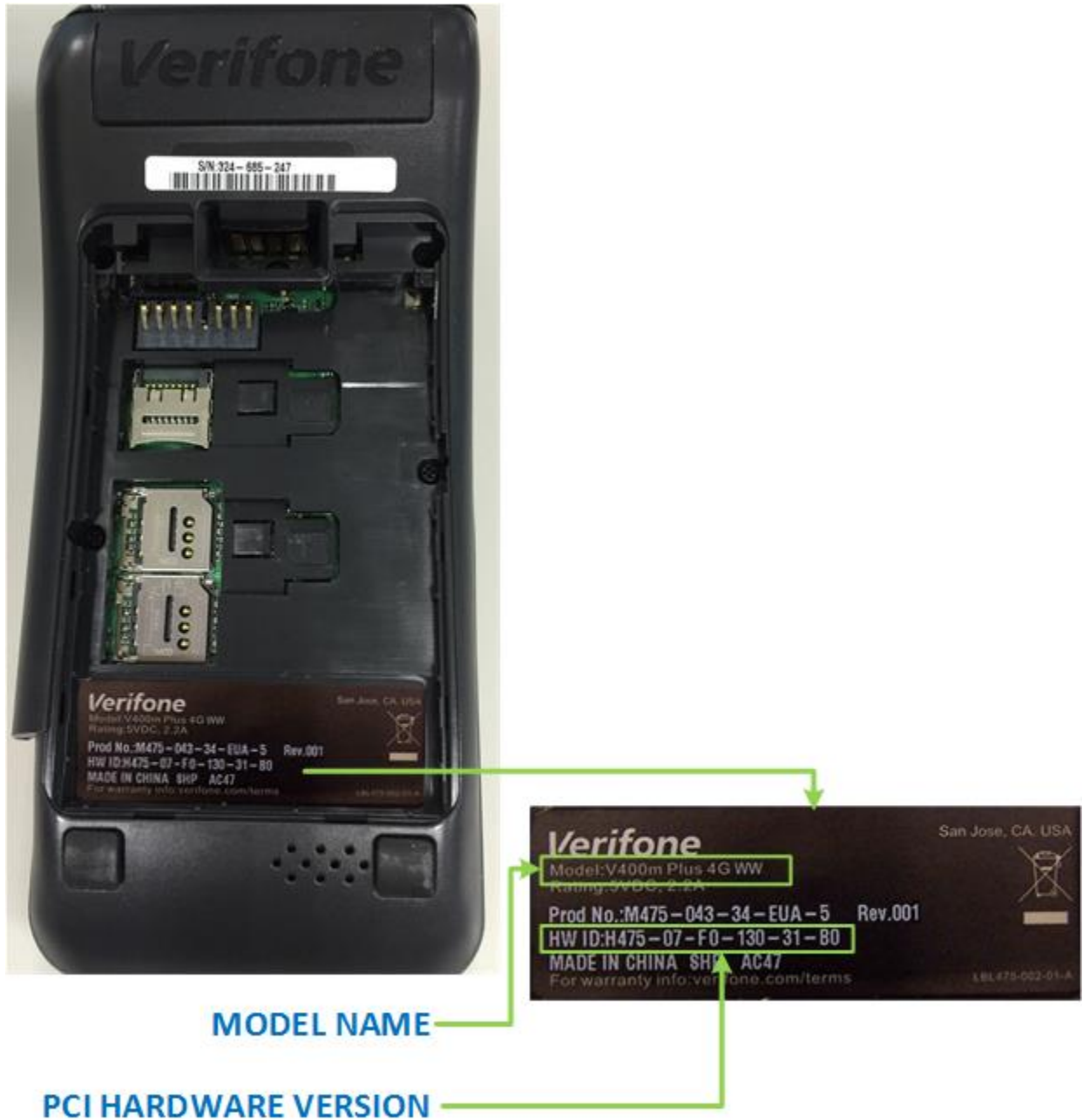
Figure 2, Hardware Identification
